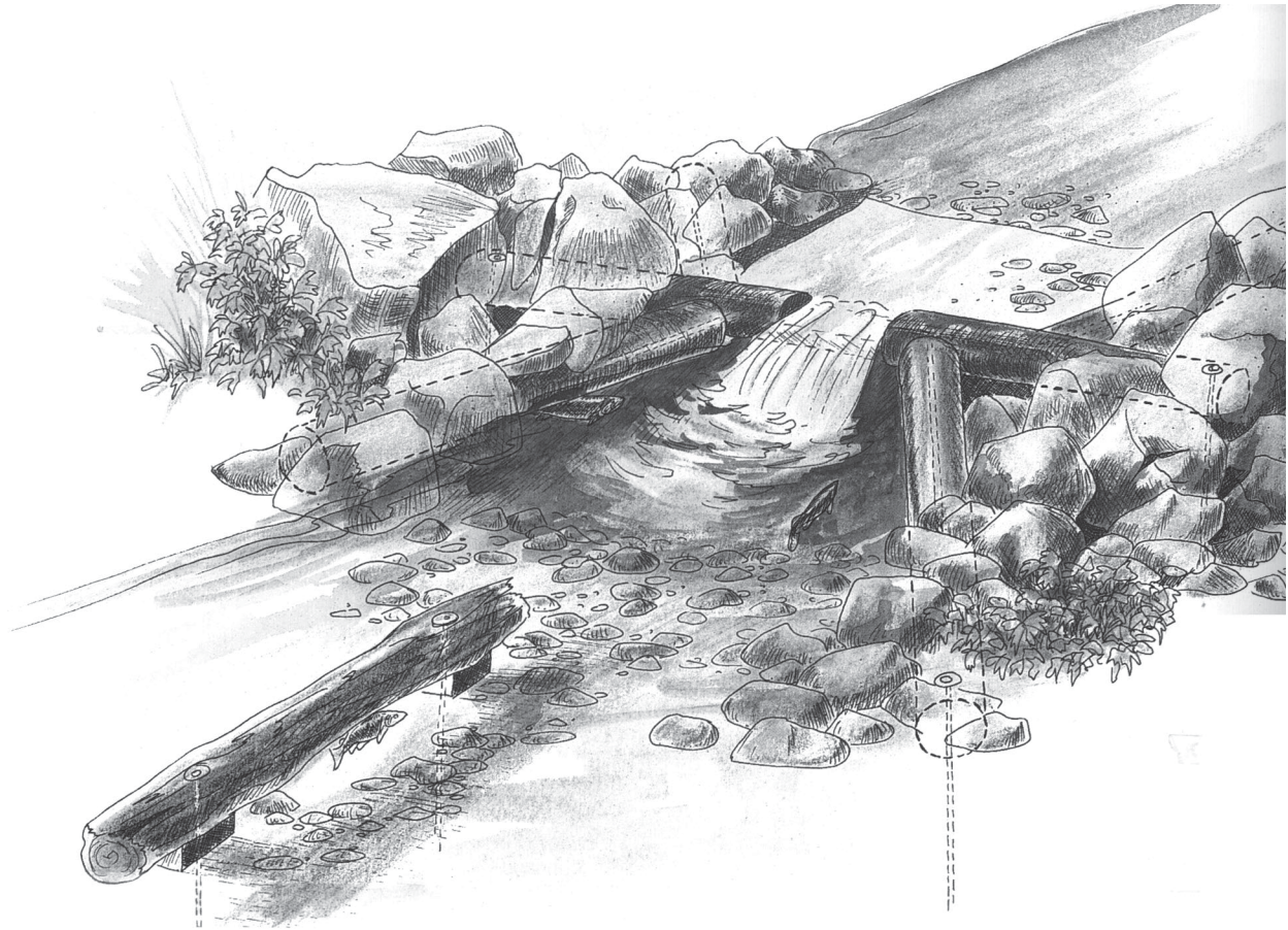
FIGURE 25. A "K-dam" creates a plunge pool that provides deepwater habitat in otherwise shallow streams.
